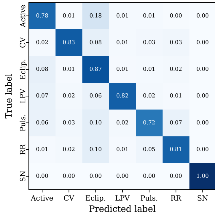
(b) Feature-based Transformer (fine-tuned)
