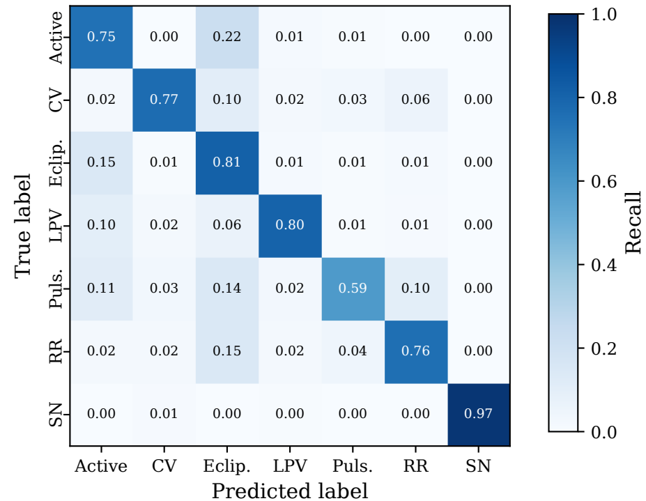
(c) E2E Transformer Small (ft)
