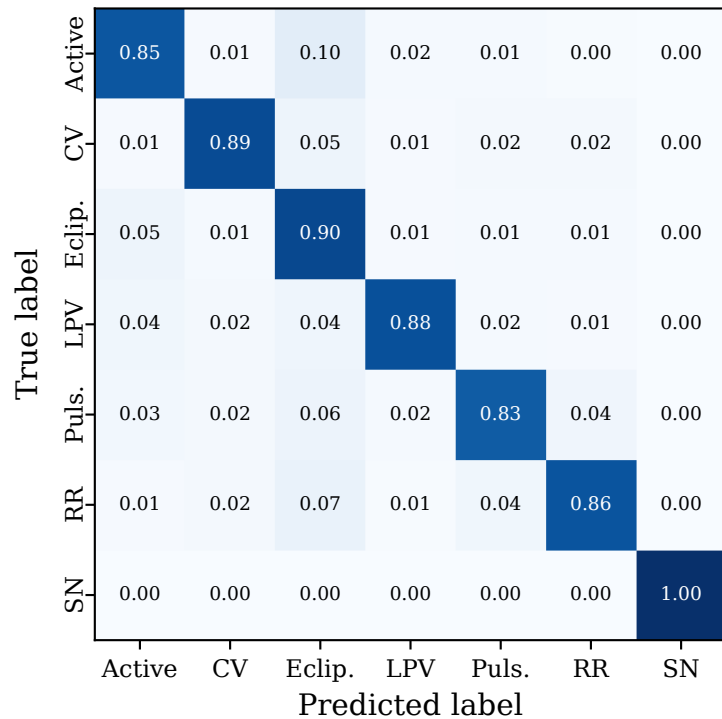
(a) Feature-based Transformer (scratch)
